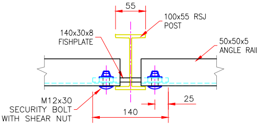
'A-A' SECTION
