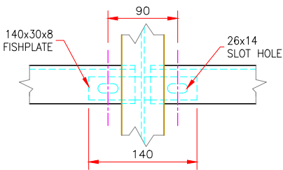
'A-A' SECTION
