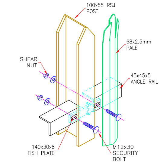
PANELS AND POST CONNECTION
