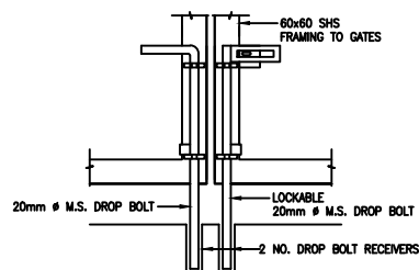
TYPICAL DROP BOLT DETAIL VIEWED FROM INSIDE
