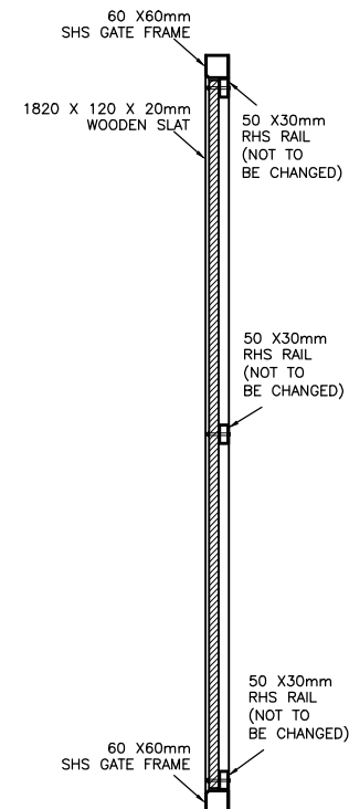
WOODEN SLAT DETAIL
