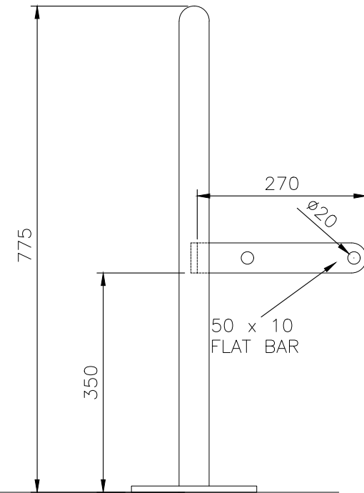
SIDE ELEVATION
