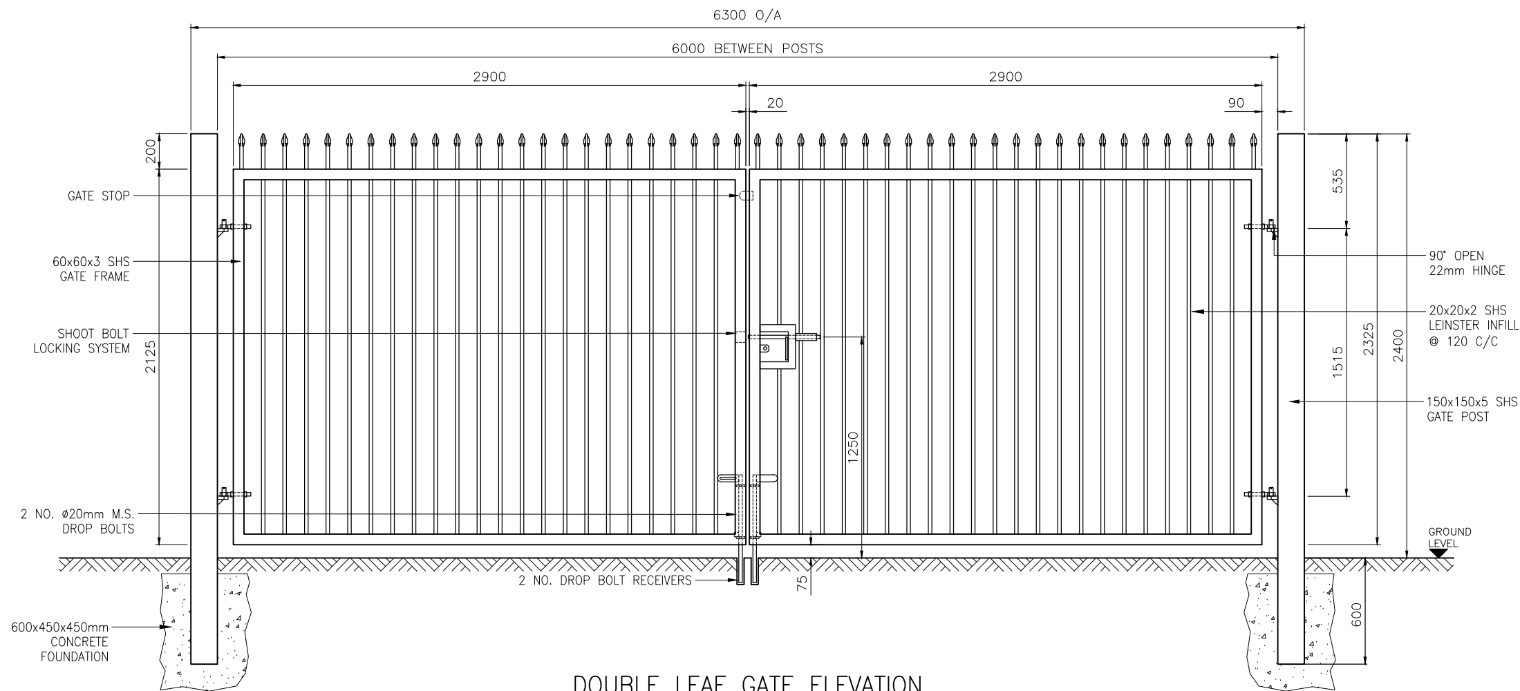
DOUBLE LEAF GATE ELEVATION VIEWED FROM OUTSIDE
