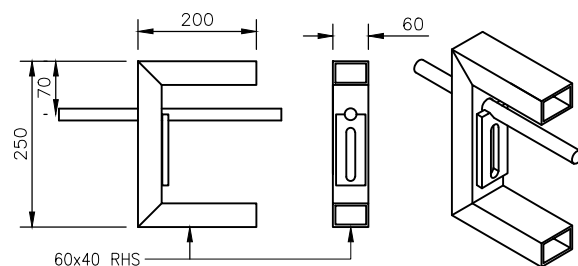
SHOOT BOLT ASSEMBLY
