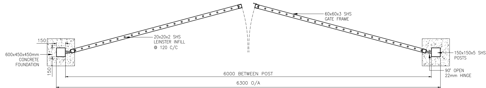
PLAN VIEW
