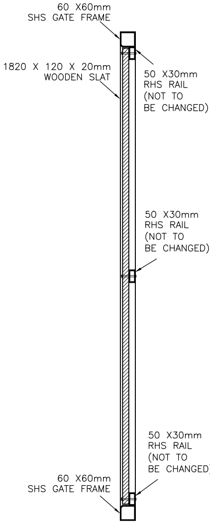
WOODEN SLAT DETAIL
