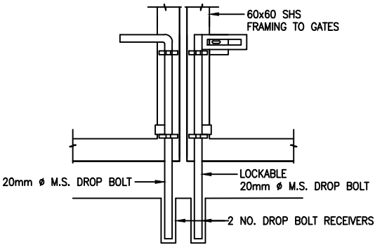
TYPICAL DROP BOLT DETAIL
