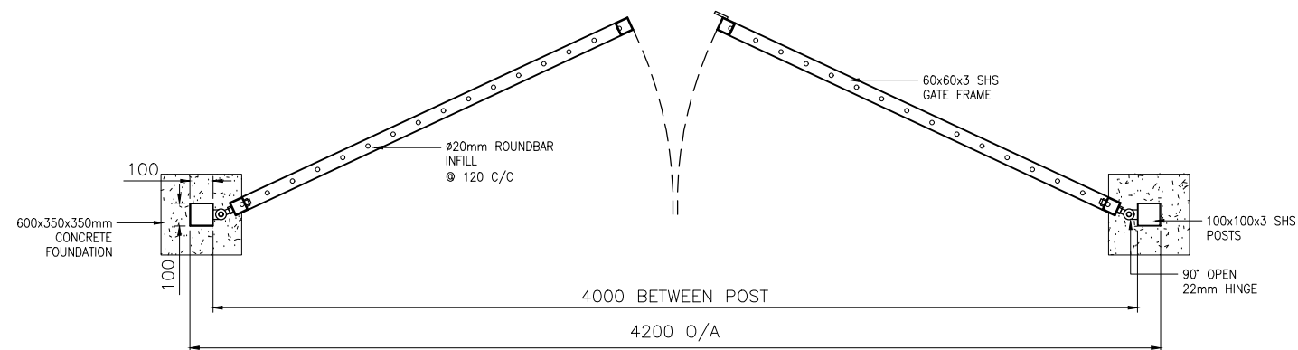
PLAN VIEW
