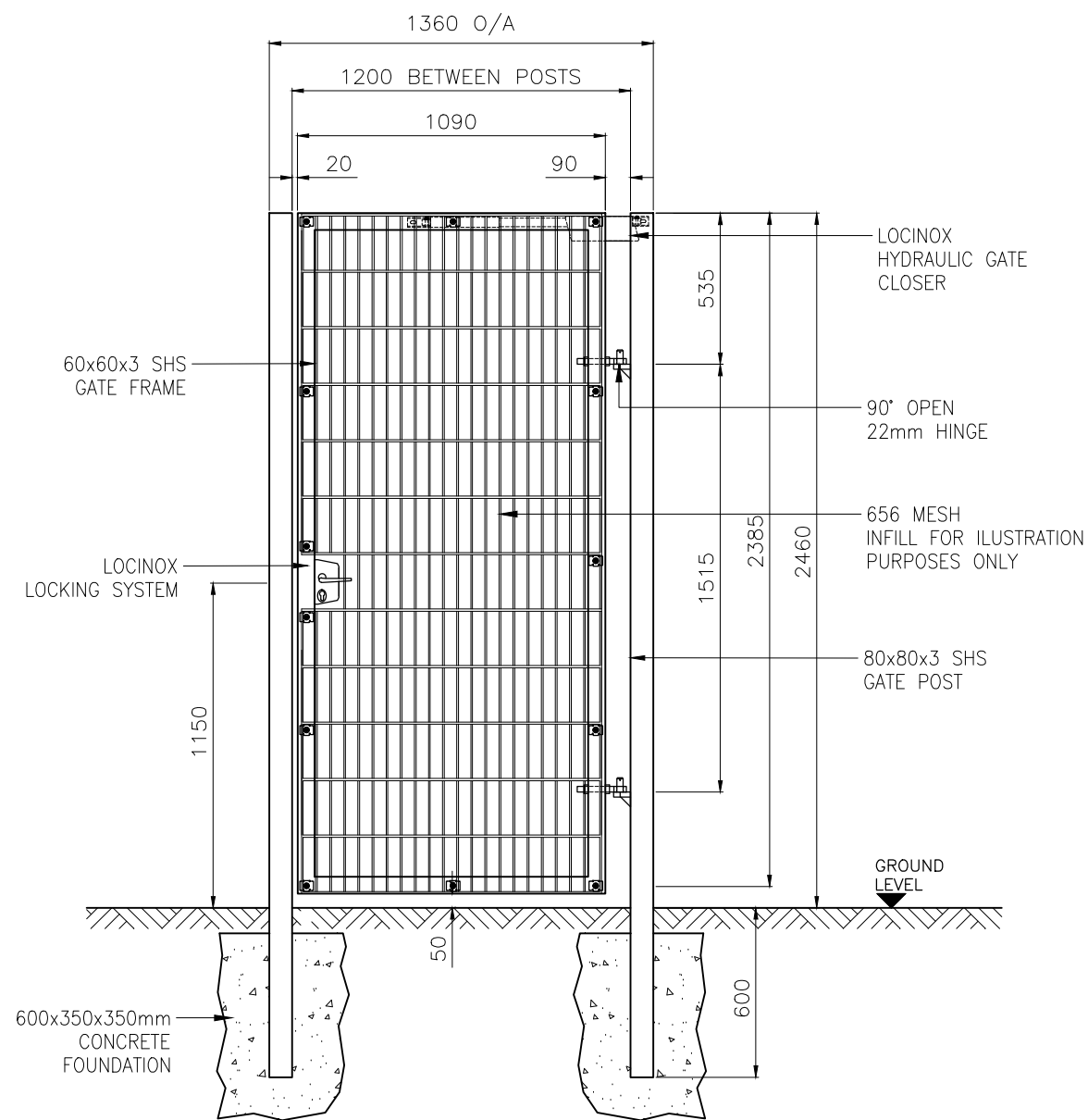
SINGLE LEAF GATE VIEW FROM OUTSIDE
