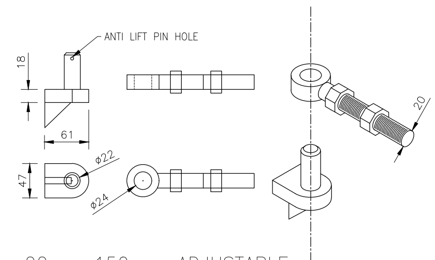
22mmx150mm ADJUSTABLE HINGE ASSEMBLY
