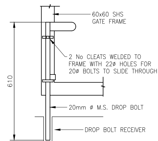
TYPICAL DROP BOLT DETAIL VIEWED FROM INSIDE
