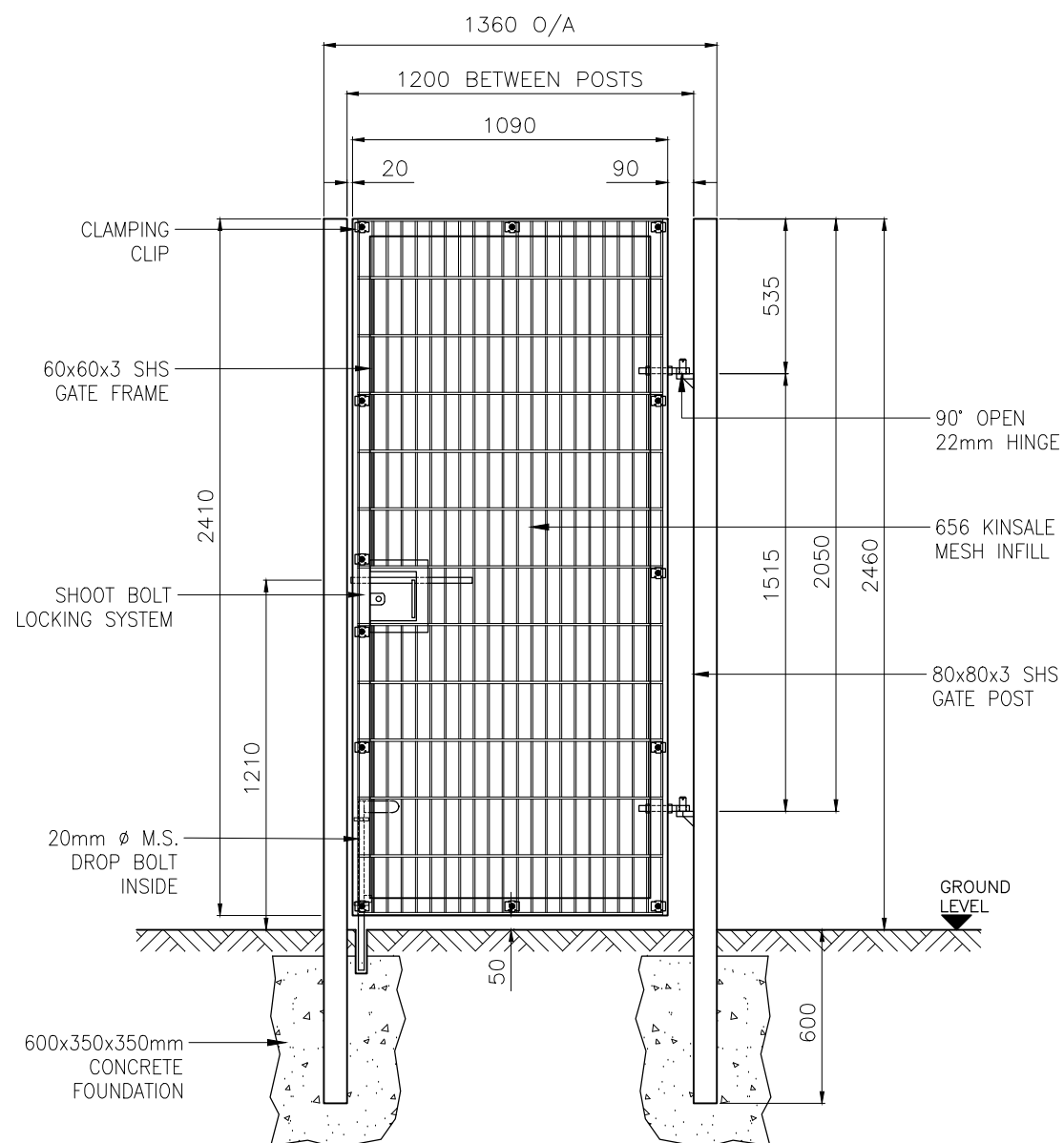
SINGLE LEAF GATE VIEW FROM OUTSIDE
