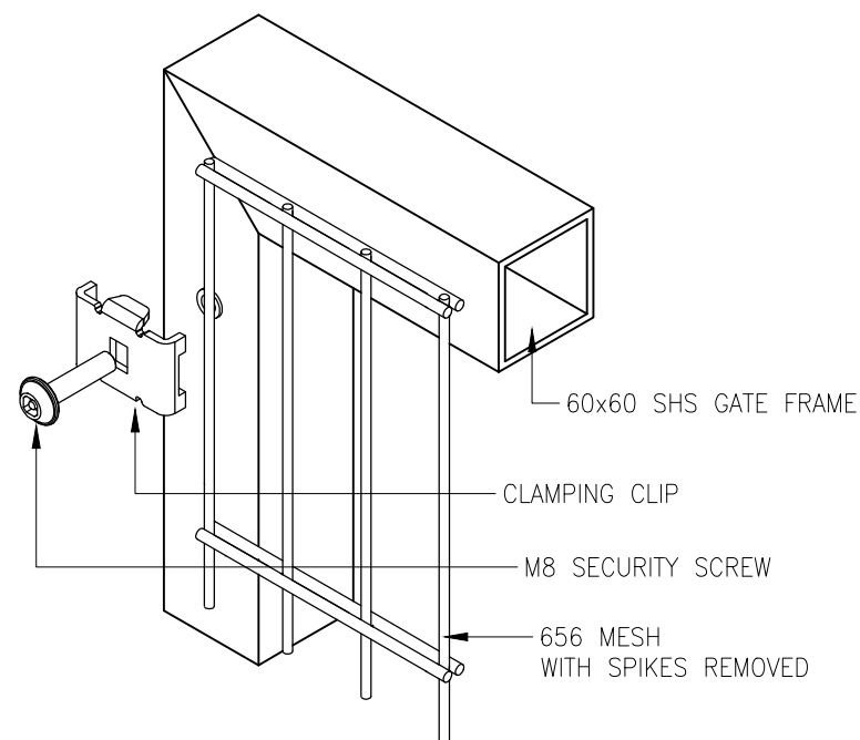
656 MESH ASSEMBLY
