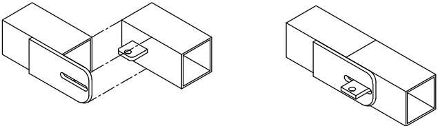
Locking Mechanism
