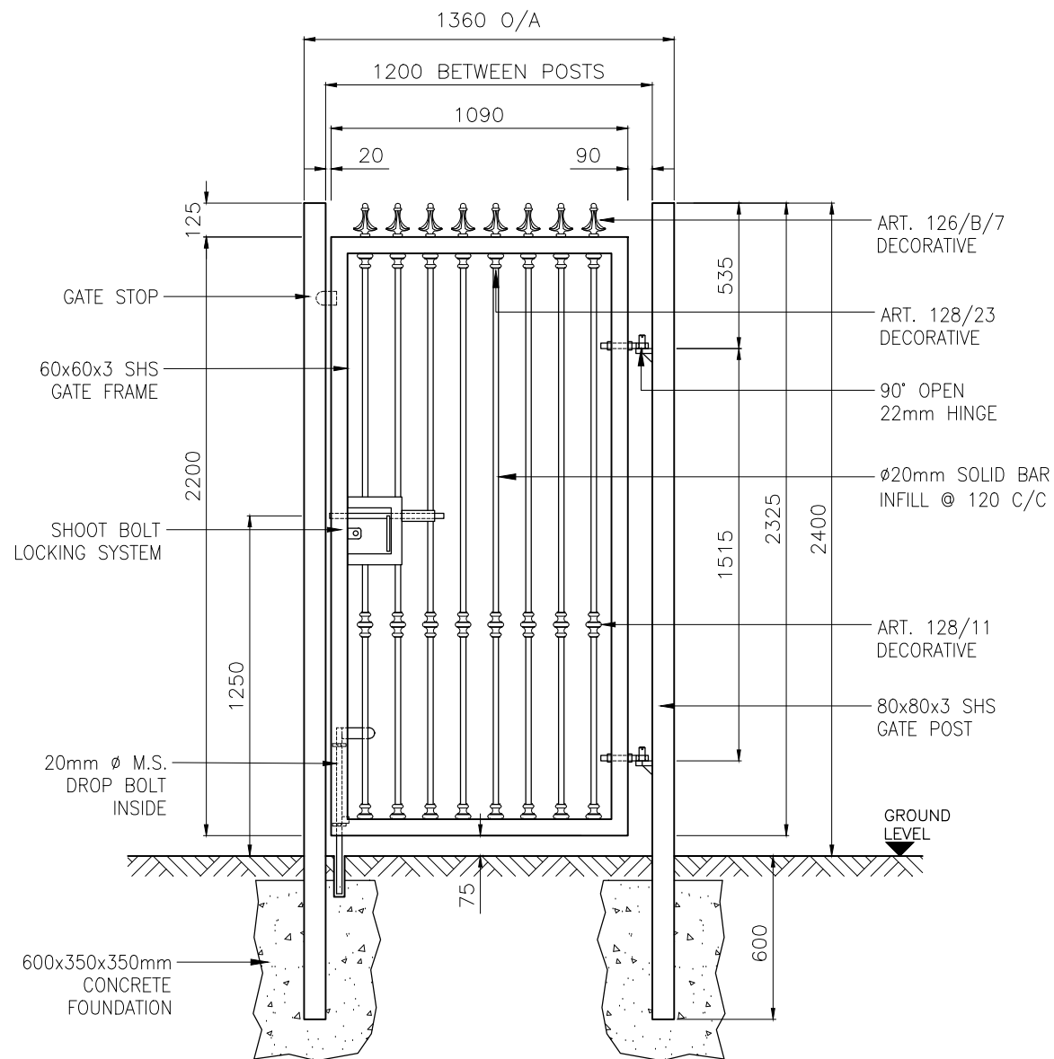
SINGLE LEAF GATE VIEW FROM OUTSIDE
