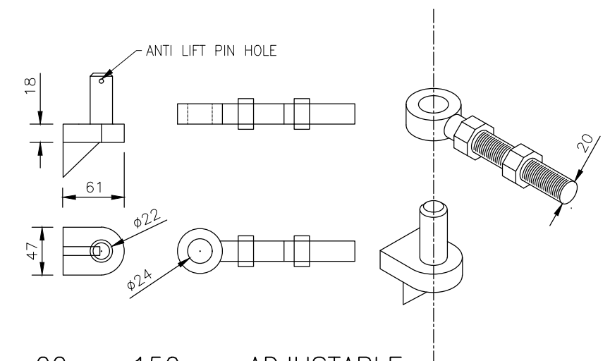
22mmx150mm ADJUSTABLE HINGE ASSEMBLY
