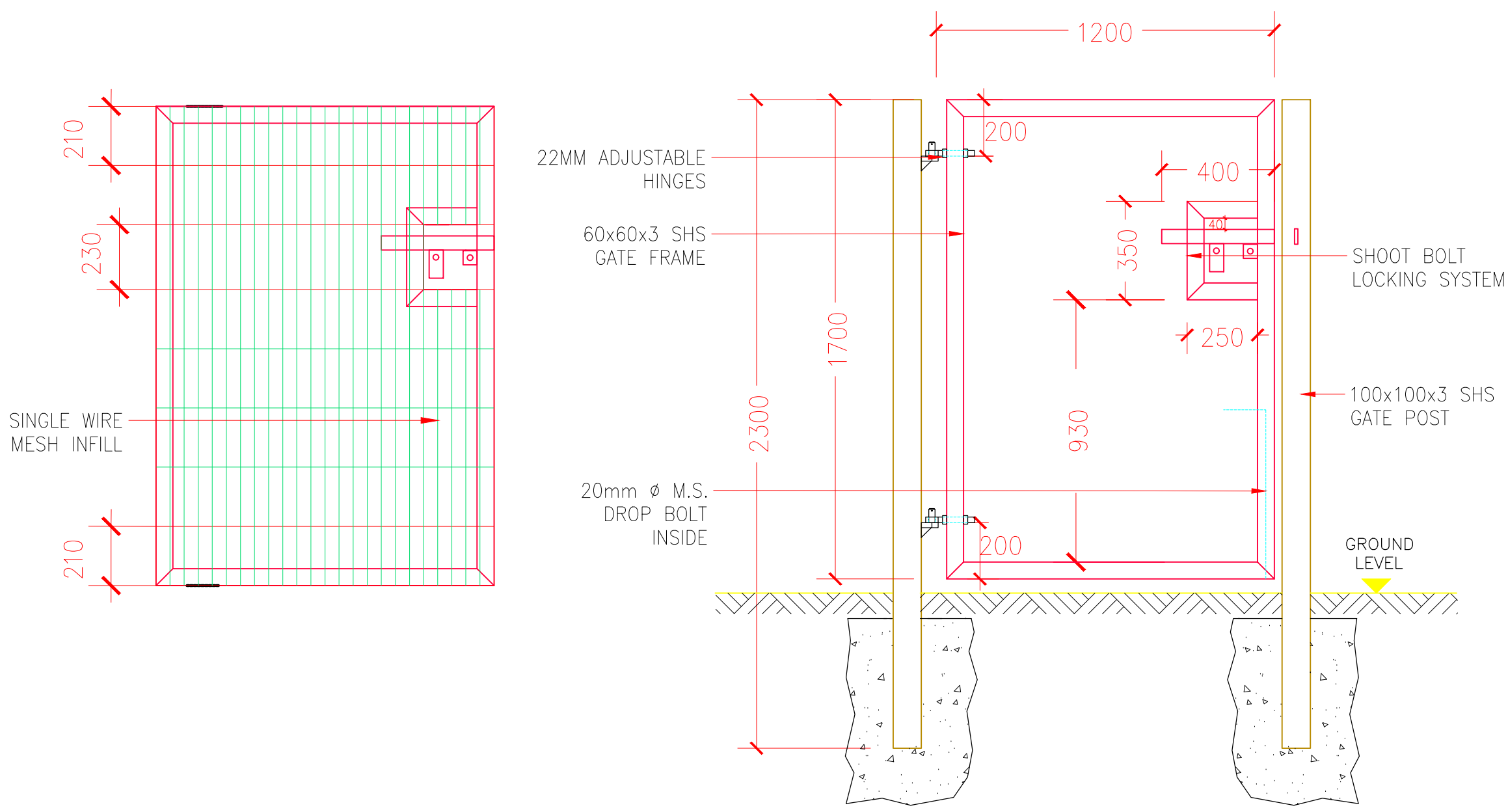
SINGLE LEAF GATE VIEW FROM OUTSIDE
