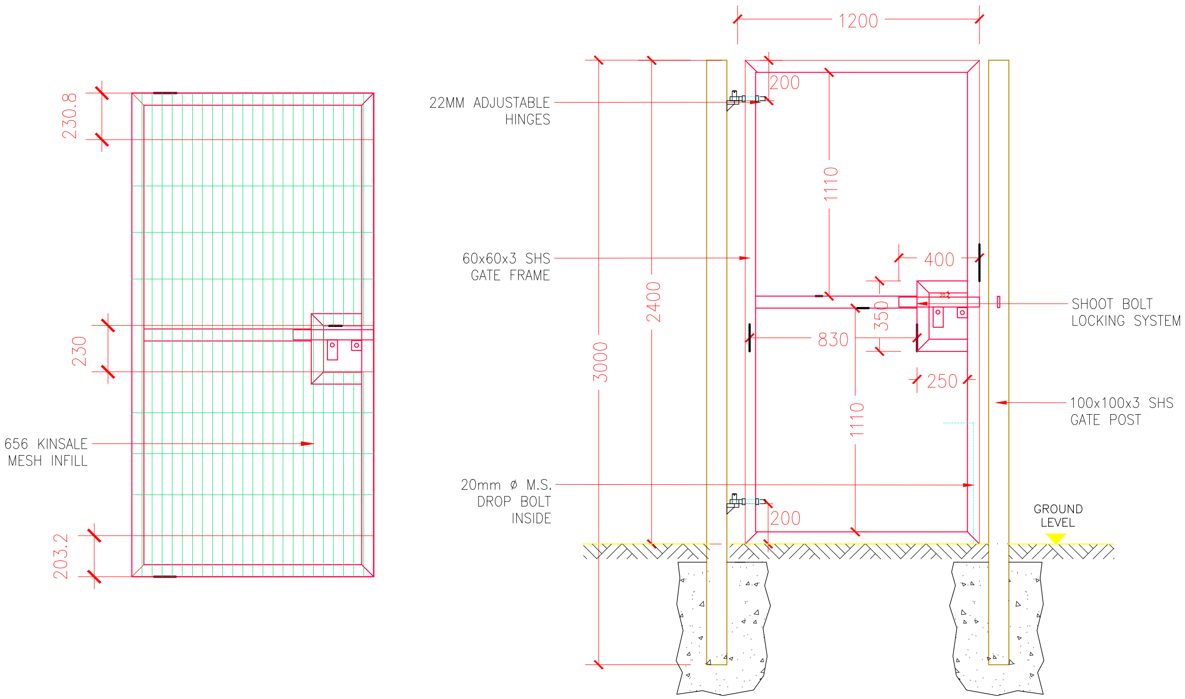
SINGLE LEAF GATE VIEW FROM OUTSIDE
