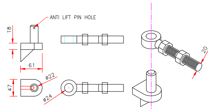
22mmx150mm ADJUSTABLE HINGE ASSEMBLY
