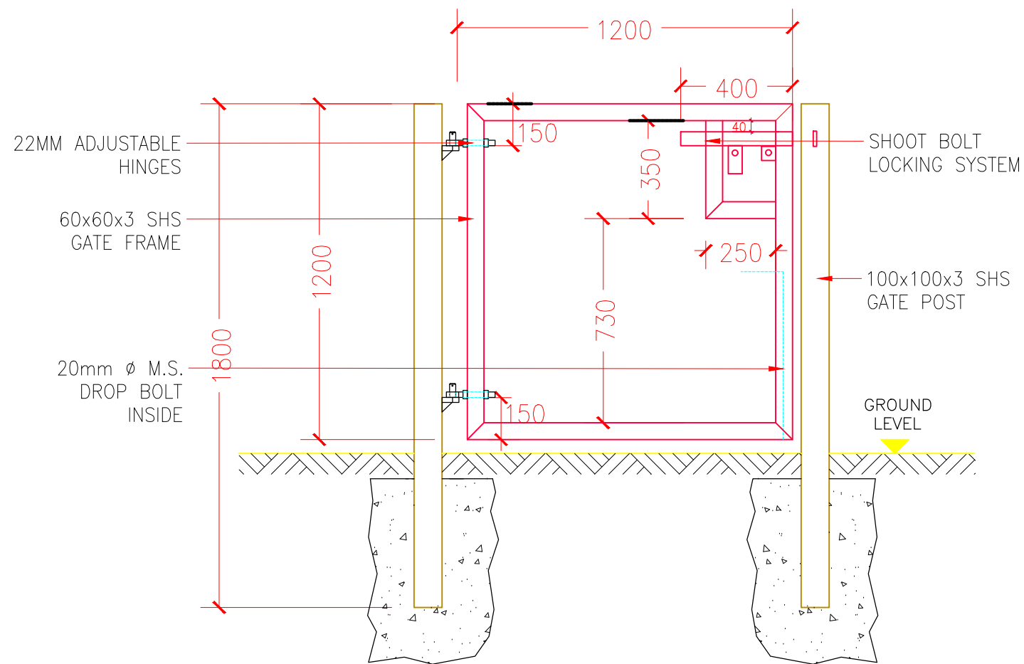
SINGLE LEAF GATE VIEW FROM OUTSIDE
