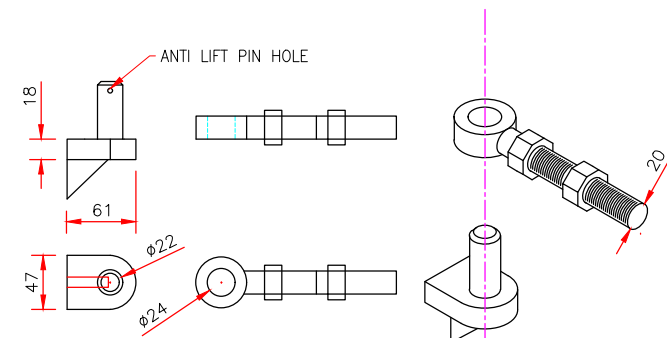
22mmx150mm ADJUSTABLE HINGE ASSEMBLY
