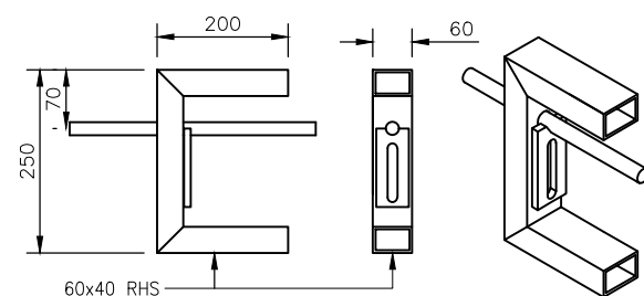
SHOOT BOLT ASSEMBLY
