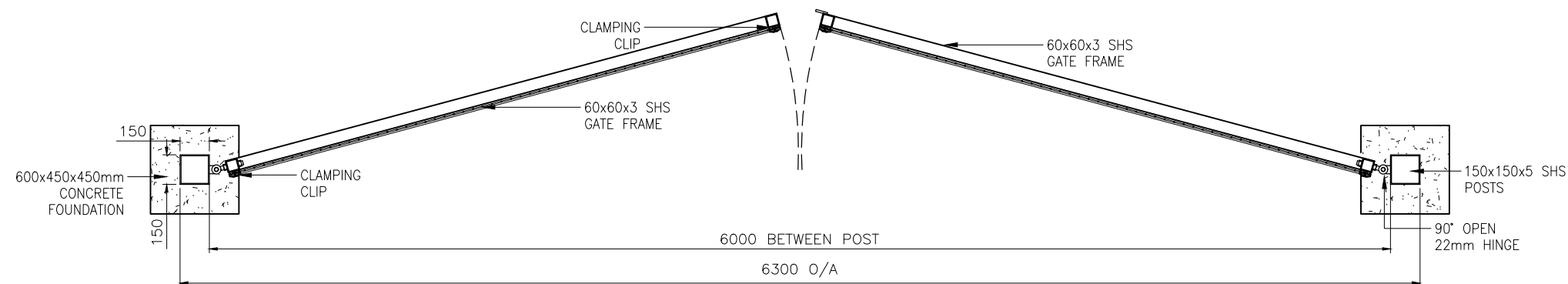
PLAN VIEW
