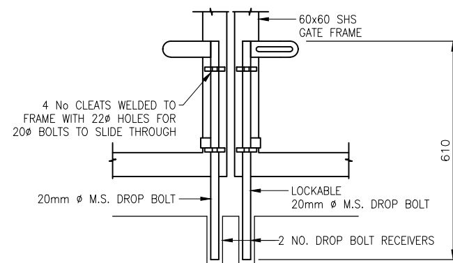
TYPICAL DROP BOLT DETAIL VIEWED FROM INSIDE
