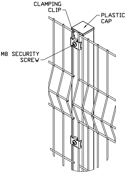
MESH FIXING DETAIL
