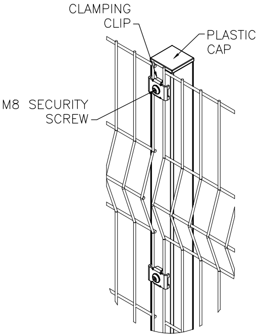
MESH FIXING DETAIL
