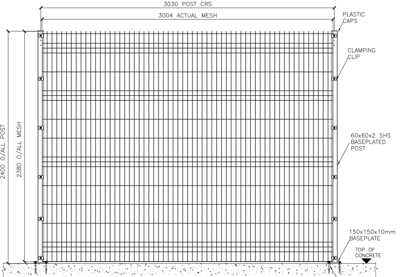
PANEL ELEVATION VIEWED FROM OUTSIDE
