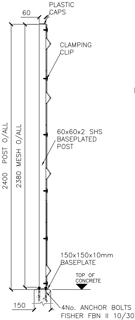
SIDE VIEW
