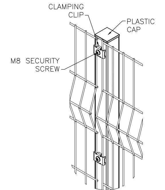
MESH FIXING DETAIL
