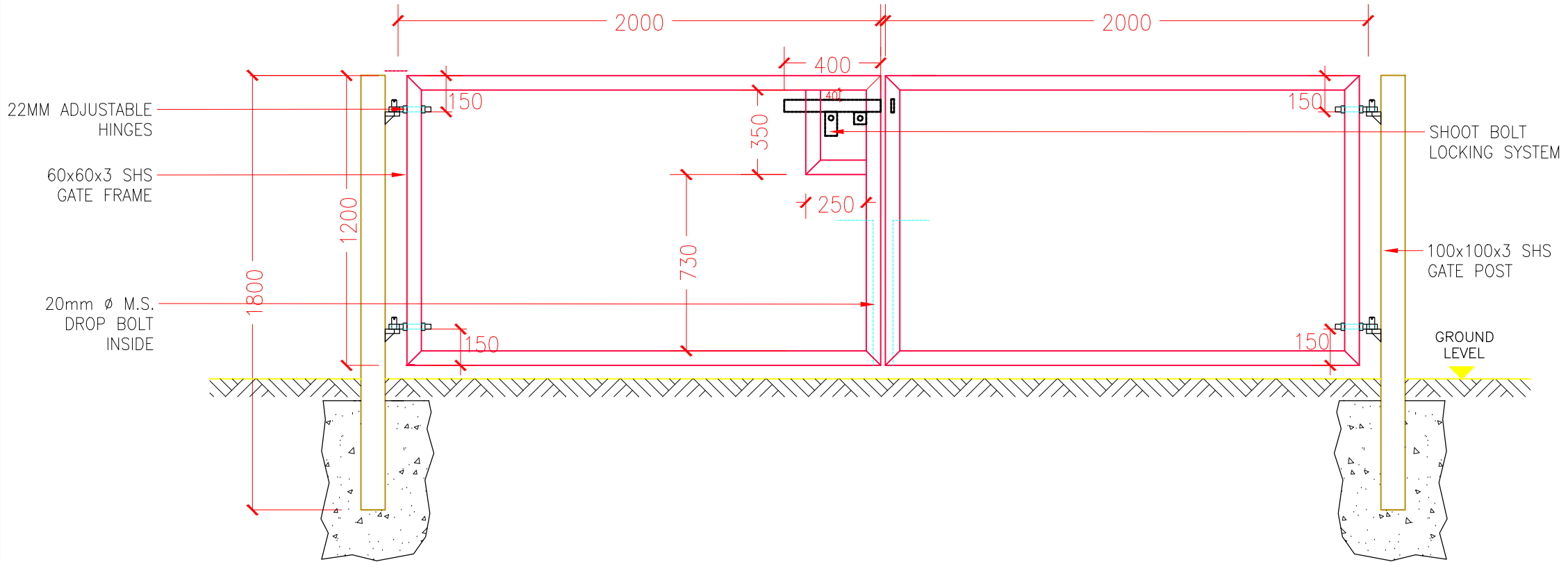
DOUBLE LEAF GATE VIEW FROM OUTSIDE
